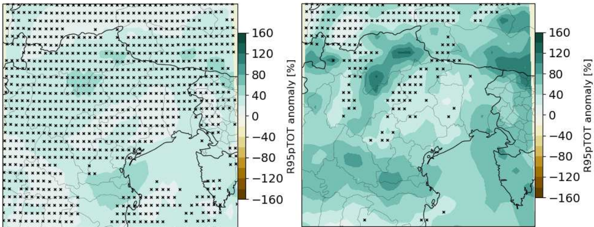
Figure 13. Geographical distribution of the cumulative precipitation larger than 95th percentile (R95pTOT) anomaly (units: percent of baseline value) in winter for the 2071-2100 with respect to the reference period 1976-2005; the left/right hand side refer to RCP2.6/RCP8.5. Crosses indicate the grid points where the model agreement is low.
