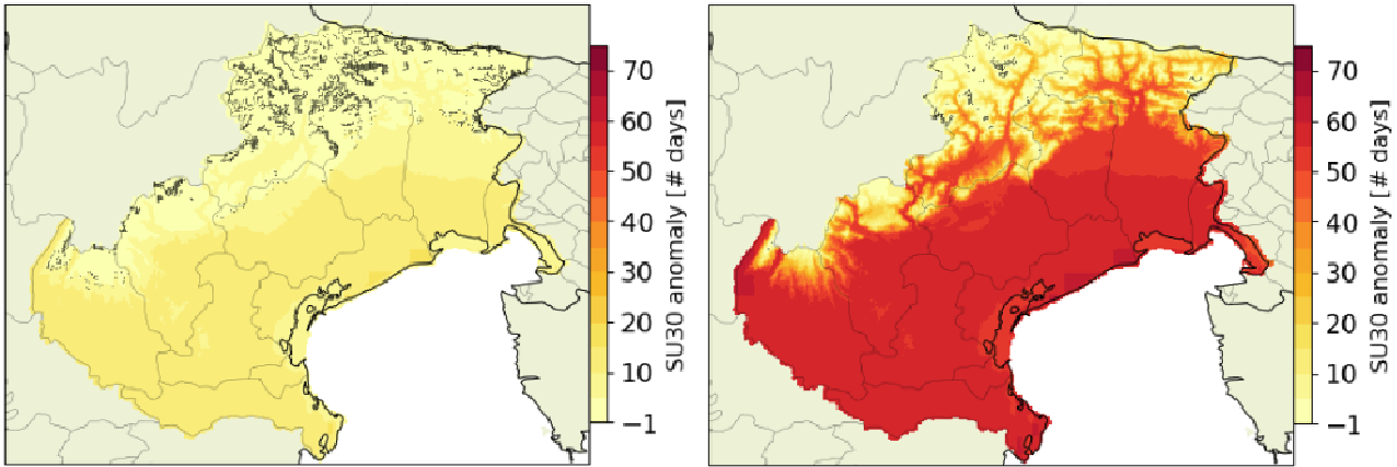
Figure 12. Geographical distribution of the summer days anomaly for the 2071-2050 with respect to the reference period 1976-2005; the left/right hand side refer to RCP2.6/RCP8.5. Crosses indicate the grid points where the models agreement is low.
