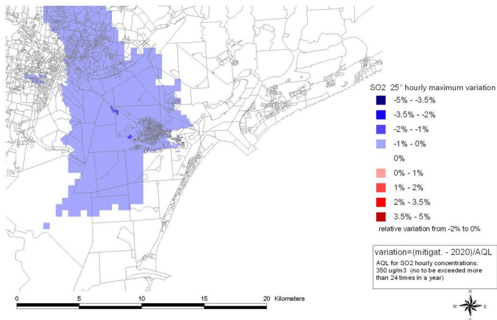
Fig. 5.2.5.7. 25th highest hourly SO 2 concentrations: percentage differences in respect to AQL, applying OPS scenario.
