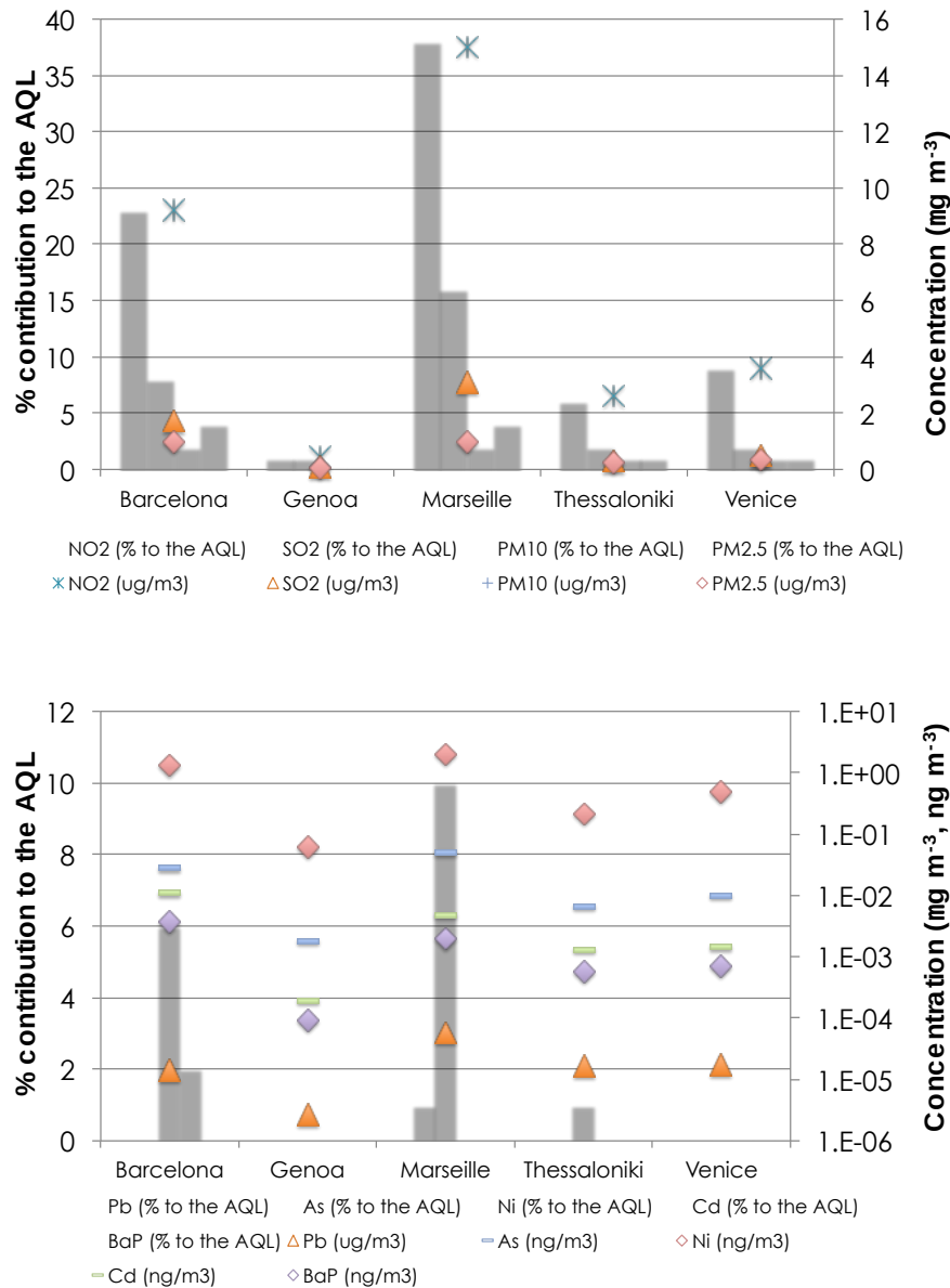
Fig. 2.3.1. Macropollutants (top) and micropollutants (bottom) domain-wide maximum percentual contribution to the annual AQL (left axis, bars) and concentrations (right axis, points) in the different study areas.
