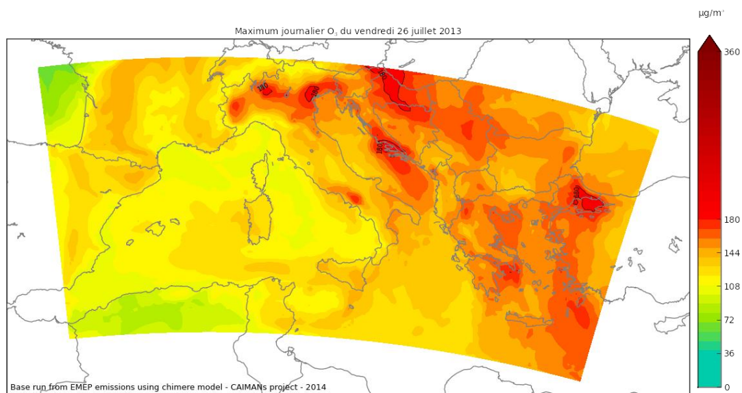
Fig. A.3.3_1: Hourly maximum O_3 during July 26 th 2013 over the CAIMANs domain with all ships using LNG as fuel
