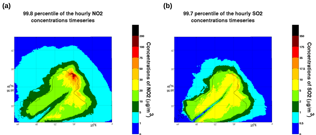
Fig. 2.2.4.1. Percentiles of the timeseries of hourly pollutant concentrations for the year 2013: (a) \text{NO}_2 and (b) \text{SO}_2 .
