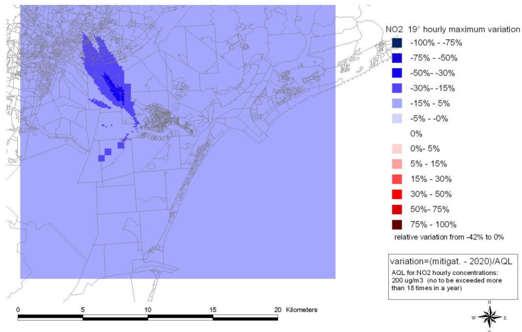
Fig. 5.2.5.5. 19th highest hourly NO 2 percentage differences in respect to AQL, applying OPS scenario.
