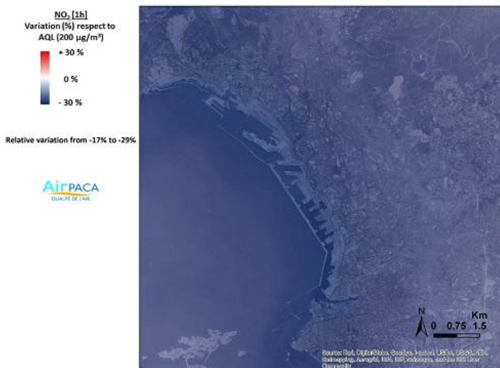
Fig. 5.2.3.2. Percentage differences in the NO 2 hourly statistics between LNG mitigation and future trend scenarios with respect to the corresponding AQL.
