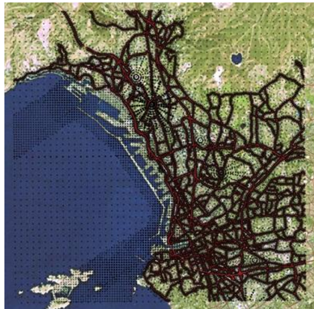
Fig. 2.2.3.1 ADMS Urban simulation area and receptor points (grey dots).
