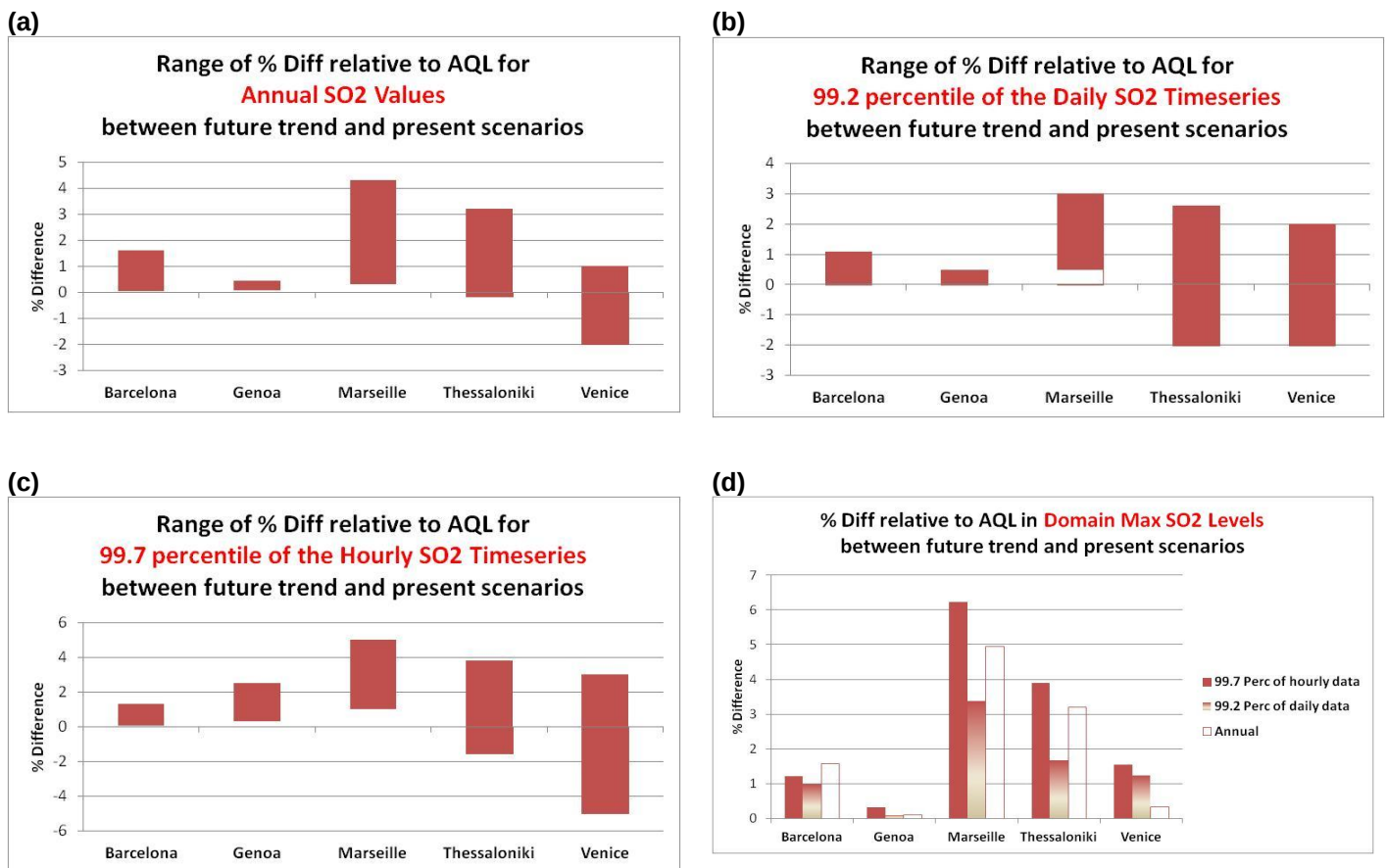
Fig. 4.2.2. (a), (b) and (c): Range of the % differences in the long-term and short-term \text{SO}_2 concentration statistics between future trend and present scenarios with respect to the corresponding AQL. (d): % differences in the domain wide maximum long-term and short-term \text{SO}_2 concentration statistics between future trend and present scenarios with respect to the corresponding AQL.
