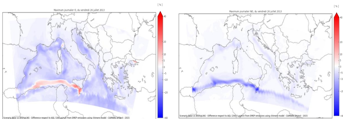
Fig. A.3.3_2: Difference between “Base scenario” and “LNG - All ships scenario” in relation to AQL for O 3 (left) and NO 2 (right) during July 26 th 2013 over the CAIMANs domain.
