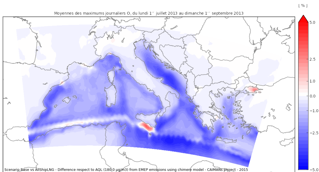
Fig. A.3.3_3: Difference between “Base scenario” and “LNG - All ships scenario” in relation to AQL for O 3 in average during summer 2013 over the CAIMANs domain.
