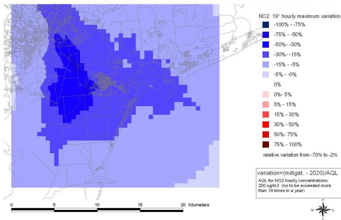
Fig. 5.2.5.2. 19th highest hourly NO 2 concentrations: percentage differences in respect to AQL, applying LNG scenario.
