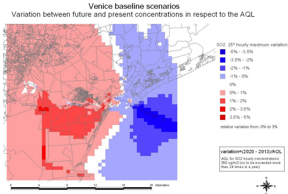
Fig. 4.1.5.2. Percentage differences between future trend and present scenarios for the 25 th highest hourly SO 2 concentration with respect to the AQL.
