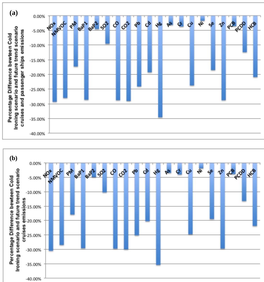
Fig. 5.2.4.1. Percentage difference between the cold ironing mitigation scenario and the future trend scenario emissions for: a) cruise and passenger ships and b) only cruise ships for the year 2025.
