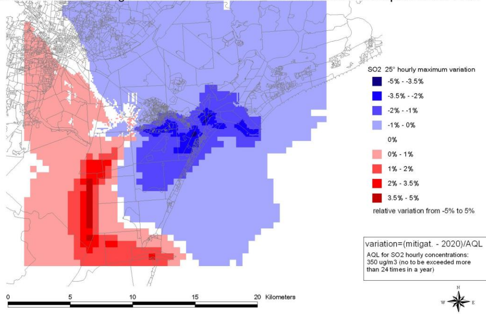
Fig. 5.2.5.13. 25th highest hourly SO 2 concentrations: percentage differences in respect to AQL, applying “Contorta” scenario.
