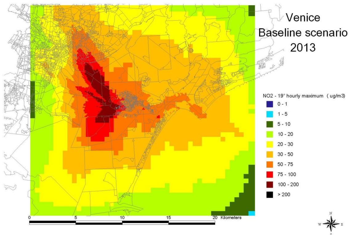
Figure 2.2.5.2. Hourly NO 2 concentrations for the reference year 2013.
