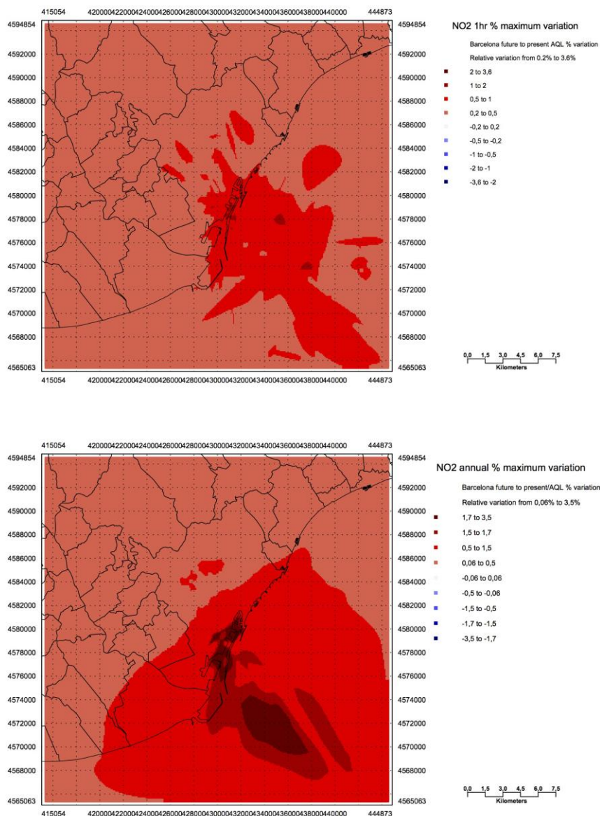
Fig. 4.1.1.1. Percentage differences relative to AQL for (top) 99.8% percentile of the 1hr NO 2 concentrations and (bottom) mean annual NO 2 concentrations between future trend and present scenarios.
