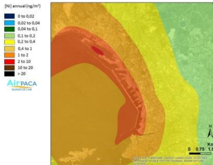
Fig. 2.2.3.4. Dispersion results (annual mean) for Ni pollutant, at present time
