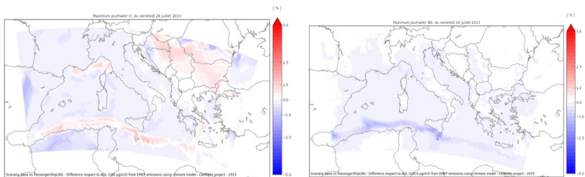
Fig. A.3.2_2: Difference between “Base scenario” and “LNG - Passenger scenario” in relation to AQL for O 3 (left) and NO 2 (right) during July 26 th 2013 over the CAIMANs domain.
