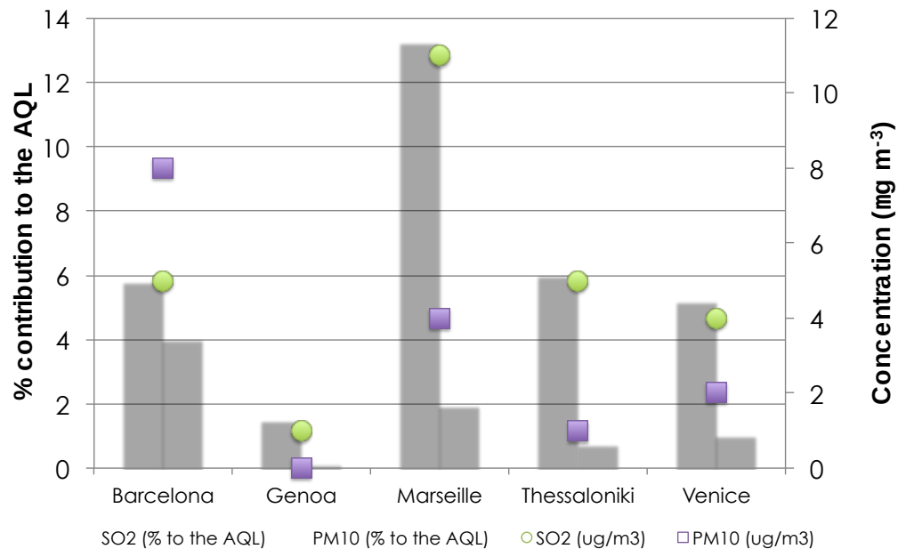
Fig. 2.3.2. SO 2 and PM 10 domain-wide maximum percentual contribution to the daily AQL (left axis, bars) and concentrations (right axis, points) in the different study areas.
