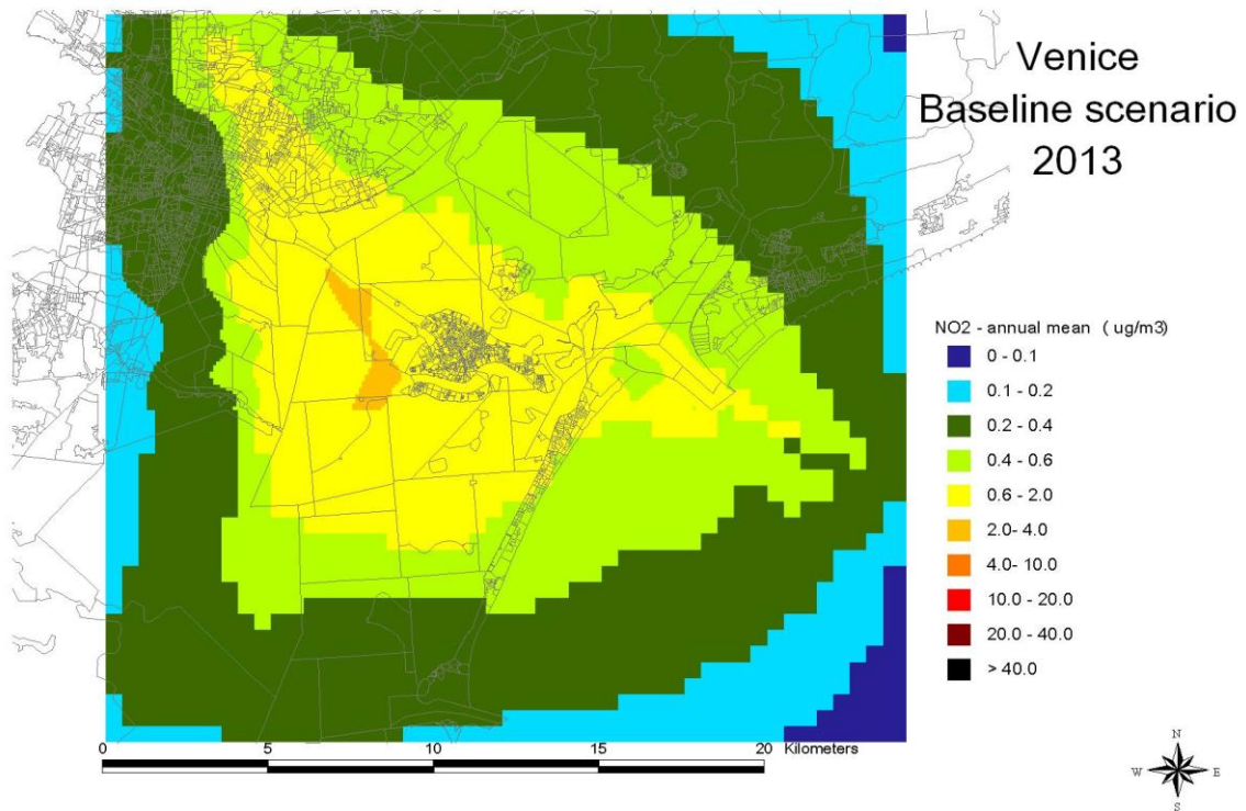
Figure 2.2.5.1. Annual NO 2 concentrations for the reference year 2013.
