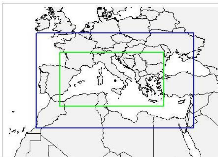
Fig. A.2.1.1_1: Extent of simulation domains.
