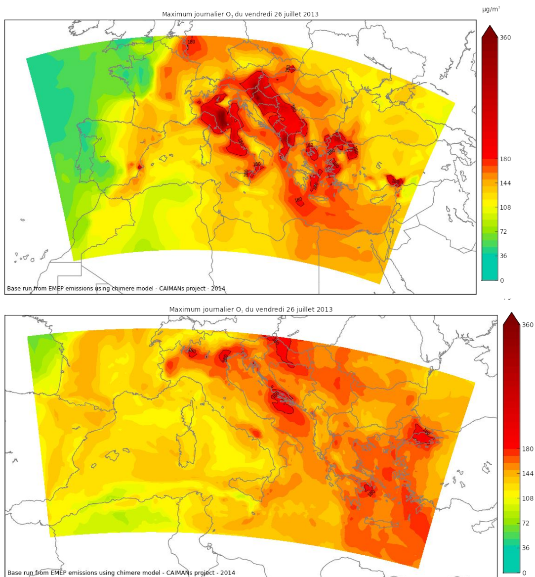
Fig. A.3_1: Hourly maximum O 3 during July 26 th 2013 over the large domain with a spatial resolution of 45km (top) and the CAIMANs domain with a spatial resolution of 15km (down).
