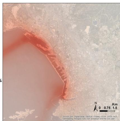
Fig. 4.1.3.3. Percentage differences in the Ni annual concentration between future trend and present scenarios with respect to the corresponding AQL (20 ng/m 3 ).
