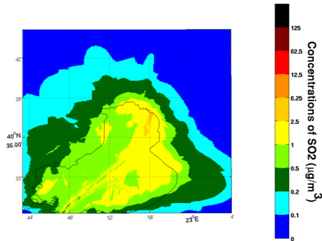
Fig. 2.2.4.2. 99.2 percentile of the timeseries of daily SO 2 concentrations for the year 2013.
