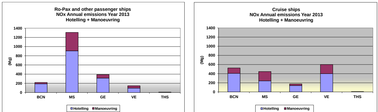
Fig. 1.3.2.2. Annual NO x emissions by Ro-pax and other passenger ships (left) and cruise ships (right) in 2013.
