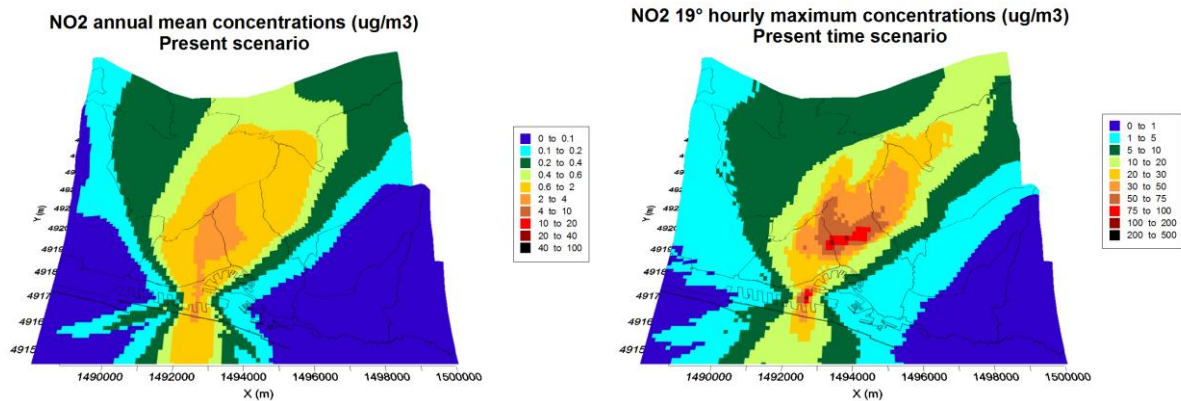
Fig. 2.2.2.3 – NO 2 concentration maps obtained with ADMS simulations. On the left side average values over the simulation period. On the right side 19 th maximum values of hourly concentrations.
