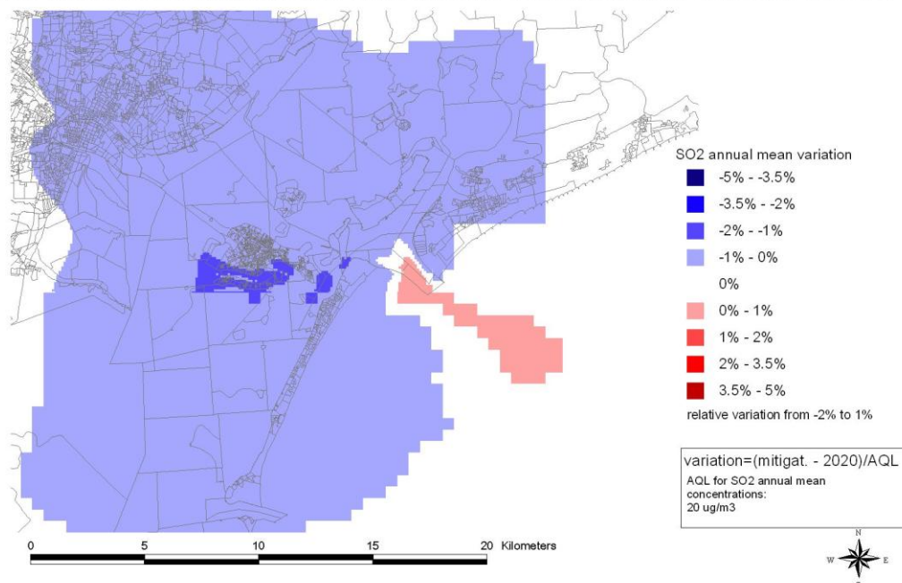
Fig. 5.2.5.18. Annual SO 2 concentrations; percentage differences in respect to AQL, applying “Punta Sabbioni” scenario.
