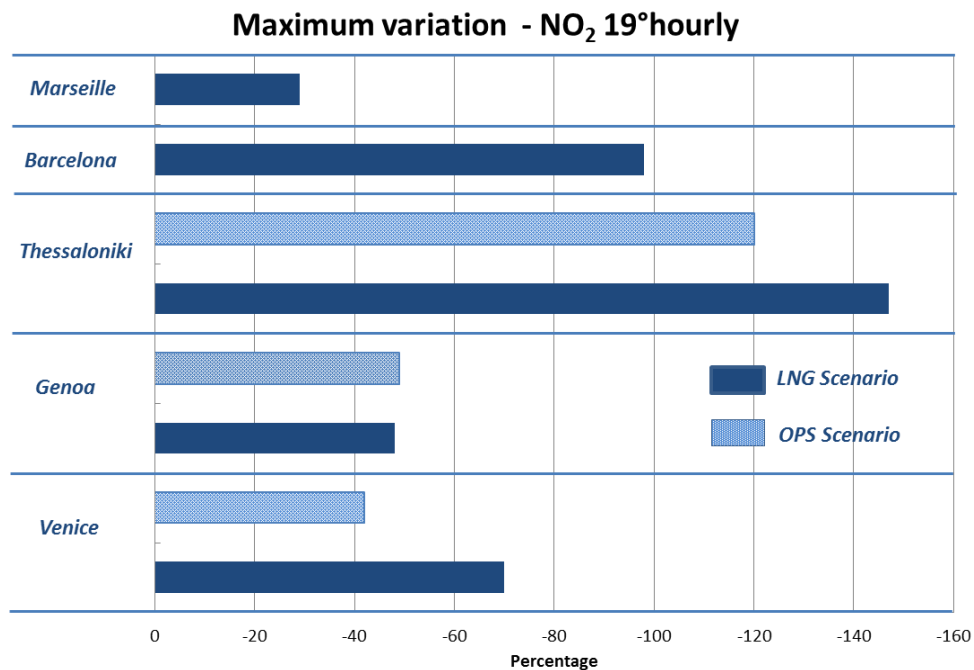
Fig. 5.3.2. Maximum variation percentage (relative to AQL) obtained for the NO 2 hourly statistics.
