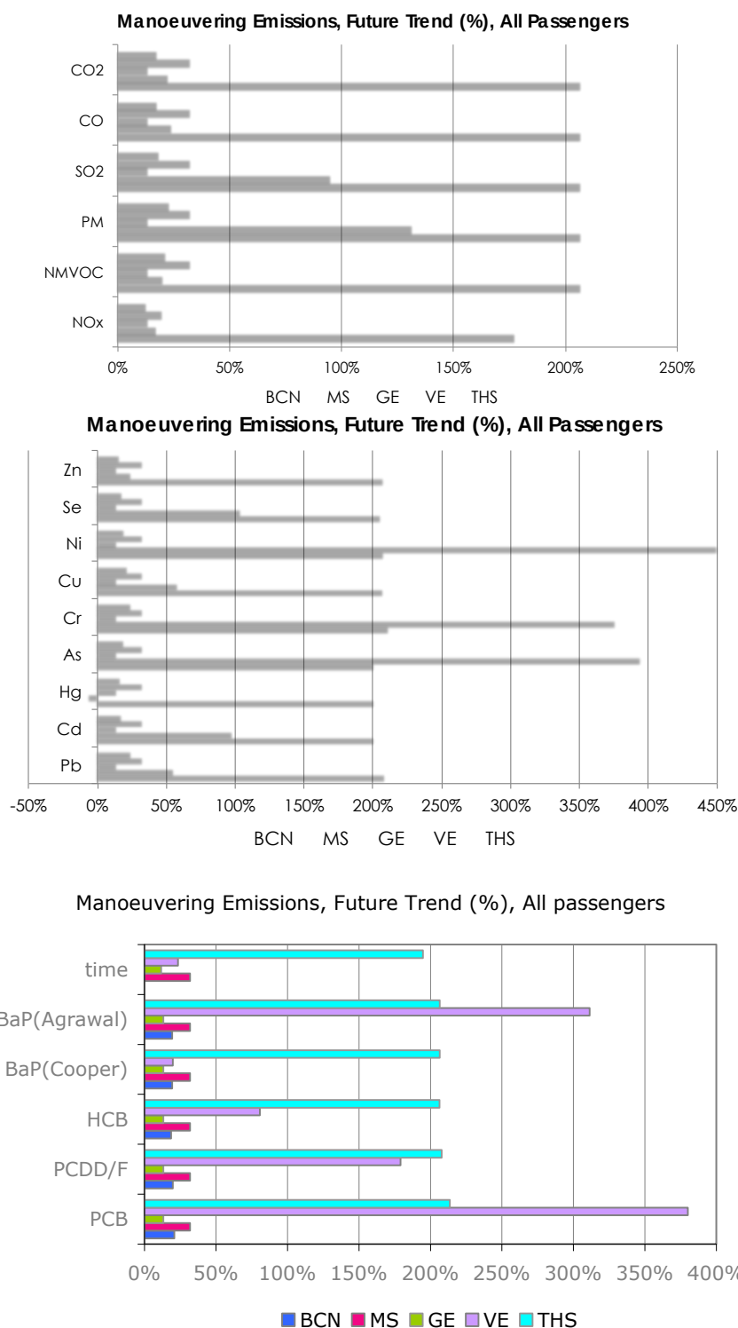
Fig. 3.3.1.5. Percentual increase in macro and micropollutant emissions for the future baseline scenarios for all passenger ships during the maneuvering phase in the five areas of study.
