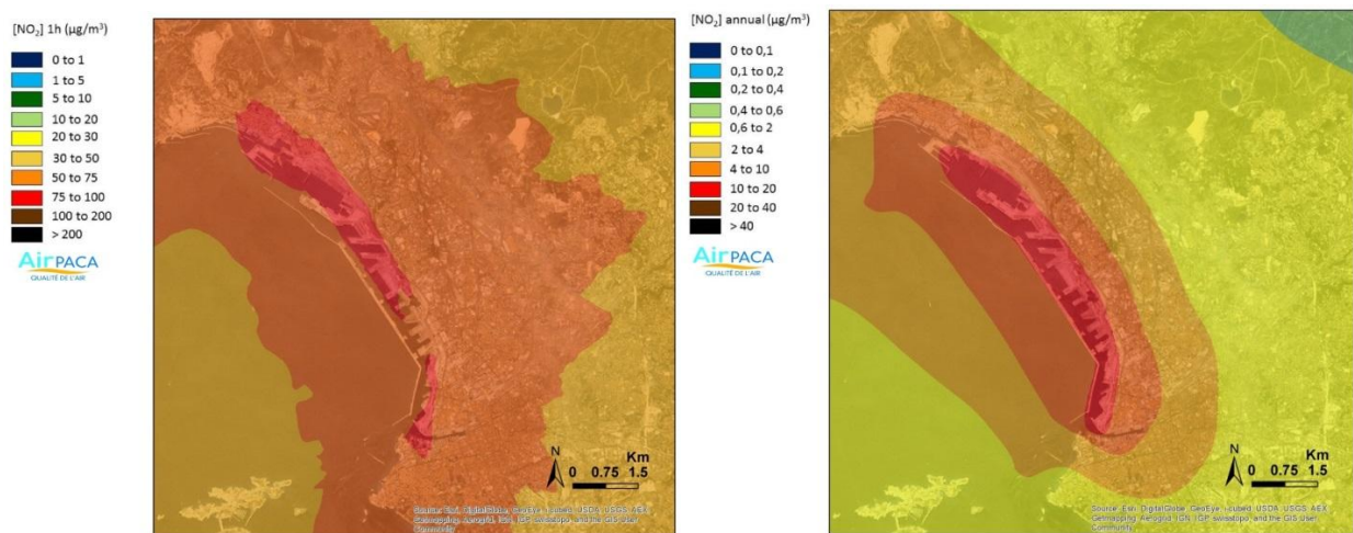
Fig. 2.2.3.2. Dispersion results for \text{NO}_2 pollutant, at present time (a) 99.8 percentile of the hourly concentrations (b) annual mean.
