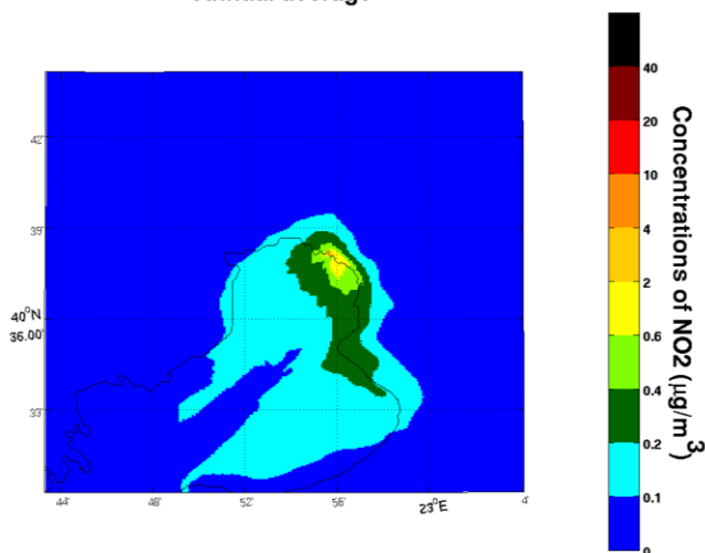
Fig. 2.2.4.3. 2013 annual concentrations of (a) NO 2 and (b) SO 2 .
