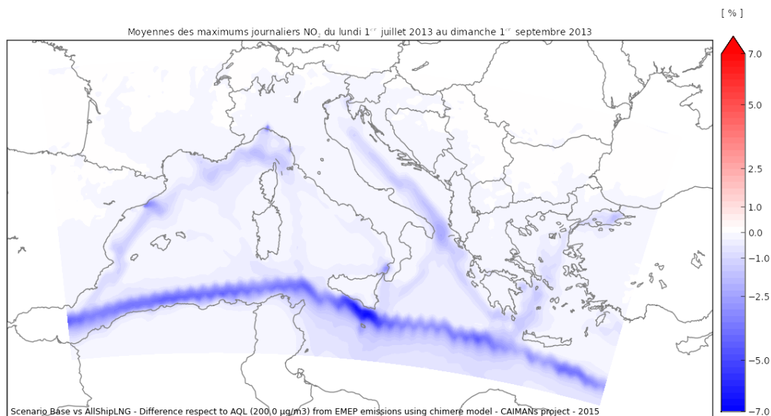
Fig. A.3.3_4: Difference between “Base scenario” and “LNG - All ships scenario” in relation to AQL for NO 2 in average during summer 2013 over the CAIMANs domain.
