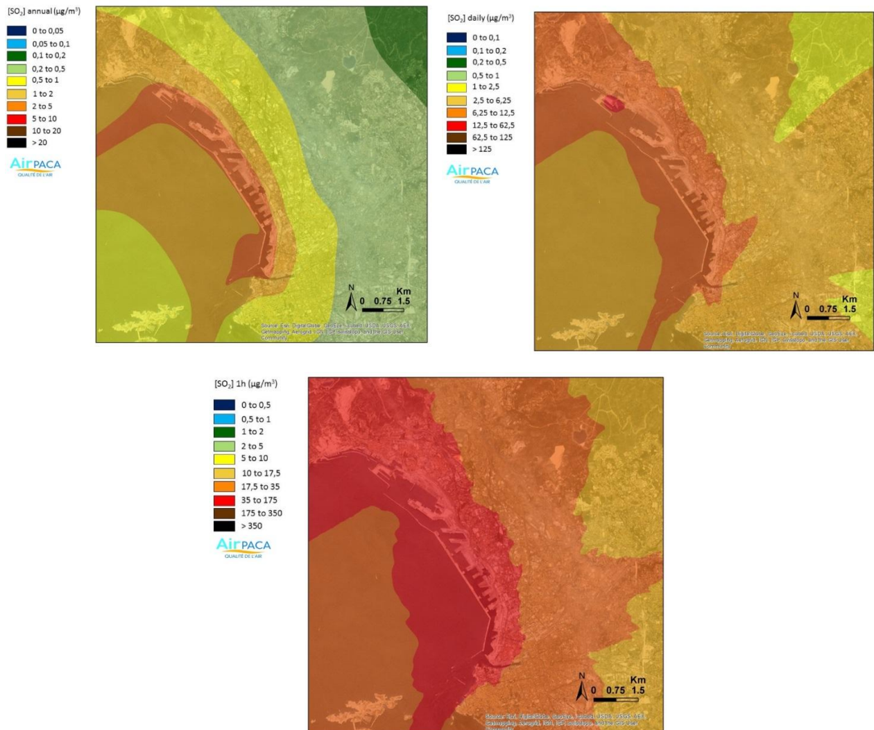
Fig. 2.2.3.3. Dispersion results for SO 2 pollutant, at present time (a) annual mean (b) 99.2 percentile of the daily concentrations and (c) 99.7 percentile of the hourly concentrations.
