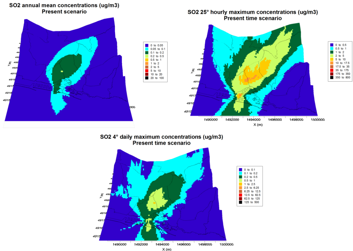
Fig. 2.2.2.4. SO 2 concentration maps obtained with ADMS simulations. On top left side average values over the simulation period. On the top right side the 25 th maximum values of hourly concentrations. The bottom figure reports 4 th daily maximum concentration values.
