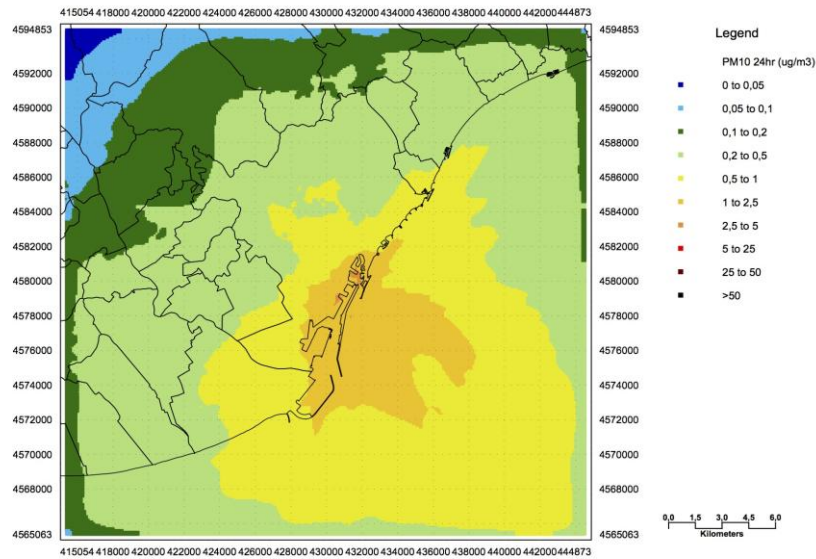
Fig. 2.2.1.2. 90.4% percentile of the 365 daily PM 10 concentrations. Reference year 2013.
