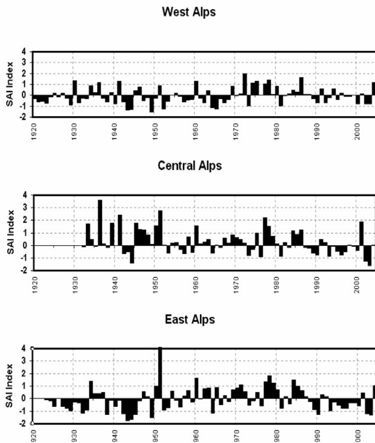
Fig. 3: SAI Index 3 sectors of the Alps
