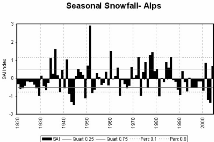
Fig. 2: SAI Index Southern Alps
